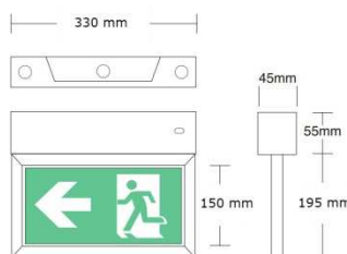
PICTOLIGHT 1P-W/C
