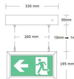
PICTOLIGHT 1P-WIRE
